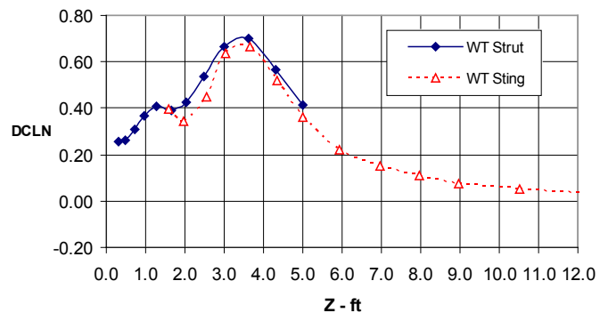
Figure 7: MK-63 Incremental Yawing Moment.
